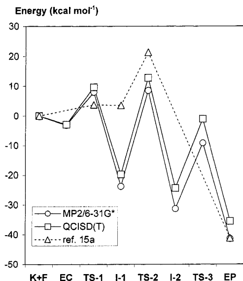
Figure 2. Proposed reaction path profile (full lines) and zwitterionic intermediate reaction path (dotted line)
