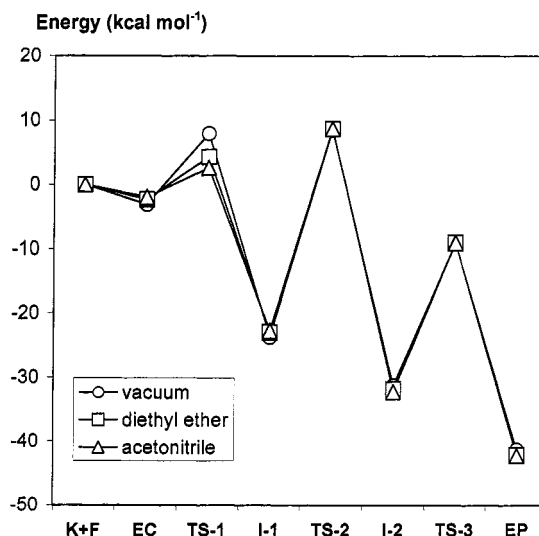
Figure 3. MP2/6-31G* + corrected ZPVE vacuum and solvent energy profiles
