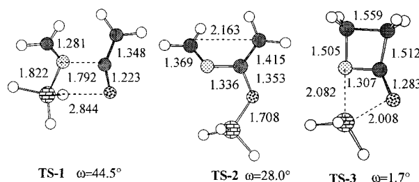
Figure 1. Fully optimized (MP2/6-31G* level) transition structures TS-1 , TS-2 , TS-3 ; bond lengths in Å; dihedral angle \omega = C=N–C=C
