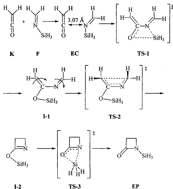
Scheme 2. Optimized intermediate and transition structures for the ketene-imine reaction
